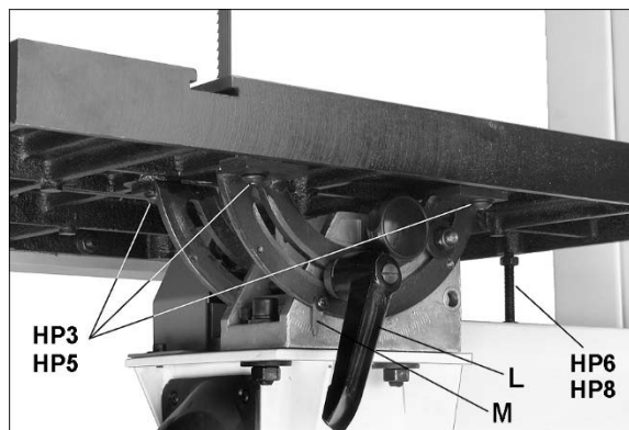
Figure 5-5: table installation
