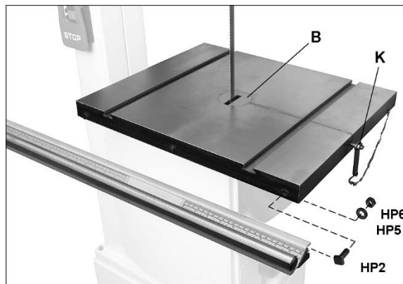
Figure 5-4: table and guide rail installation
