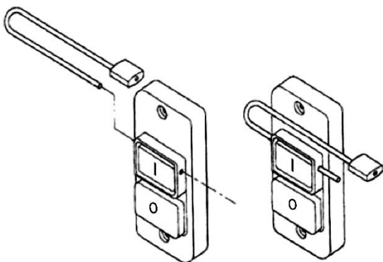
Figure 8-1: switch lockout
