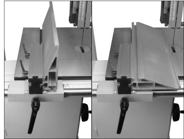
Figure 7-1: fence positions
